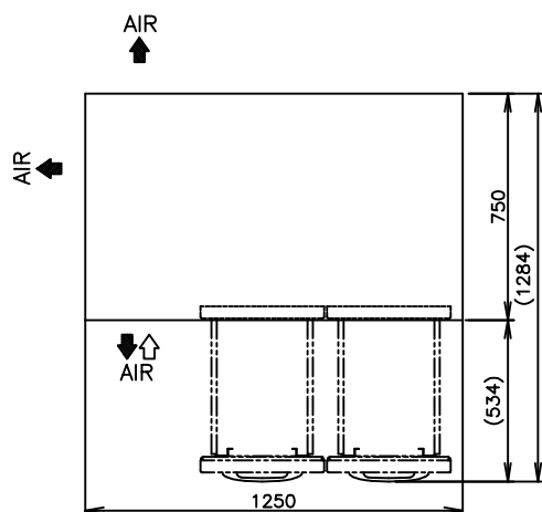
VIEW A (1/10)
