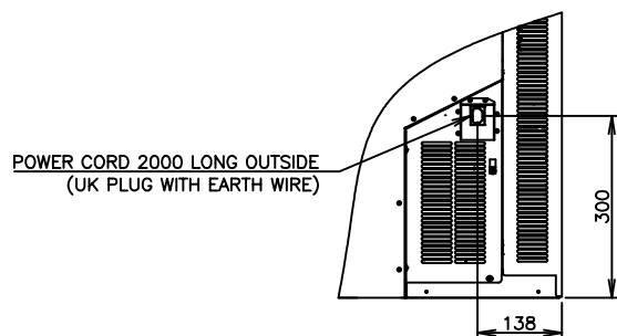
VIEW A (1/10)
