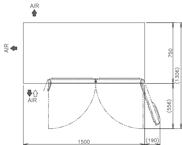
VIEW A
