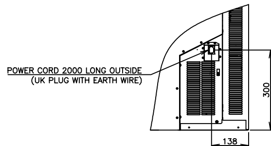
VIEW A (1/10)
