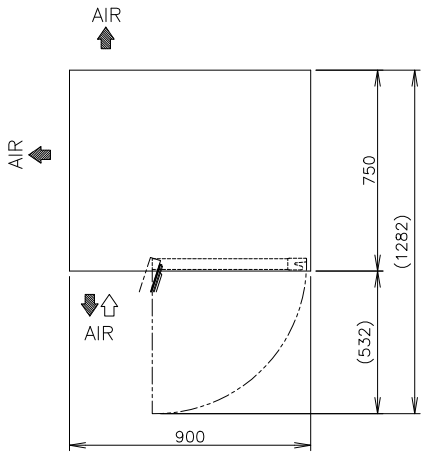
VIEW A(1/10)
