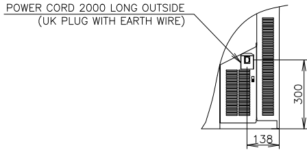
VIEW A(1/10)
