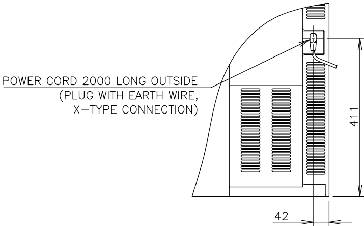
VIEW A(1/10)
