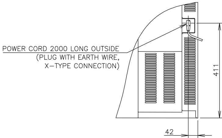
VIEW A
