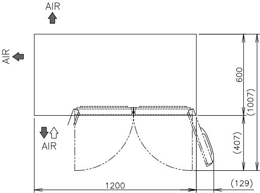
VIEW A
