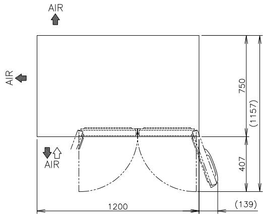
VIEW A
