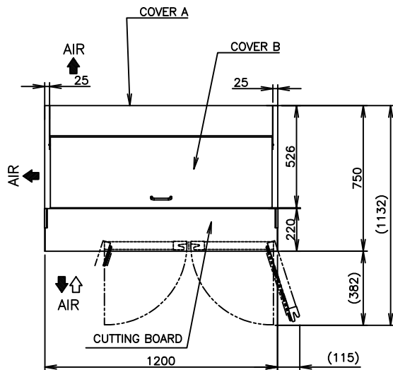
VIEW A
