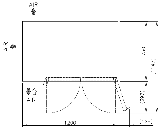
VIEW A
