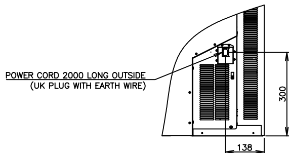
VIEW A (1/10)
