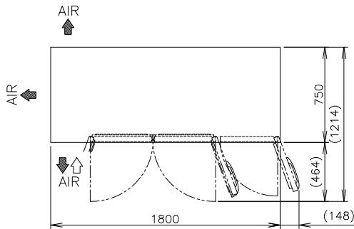
VIEW A
