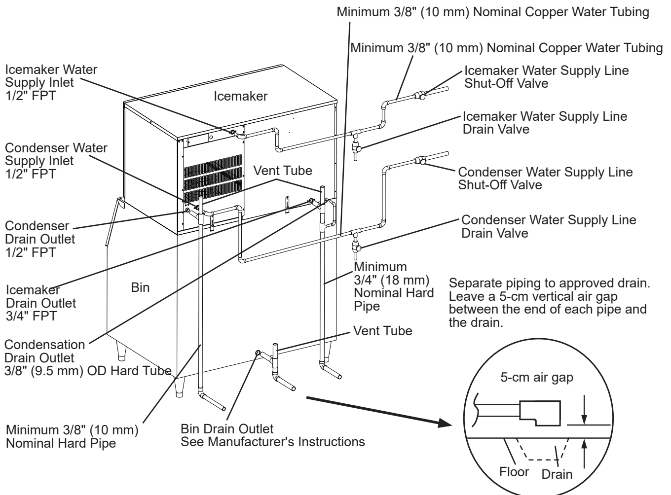
KM-590DWJ/KM-590DWJ-S Connection to an Open Drain System
