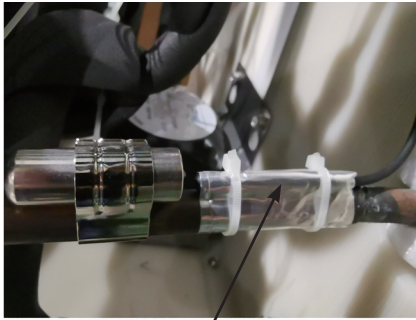
The tail distance of Evap. Sensor is about 35mm from the foaming body
