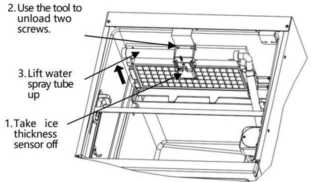
[SRM-45/60/80A]
