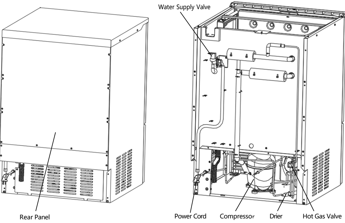
Rear View
