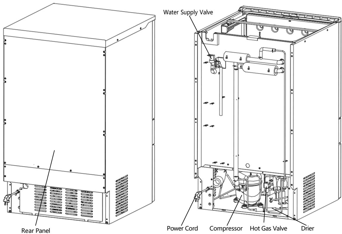
Rear View
