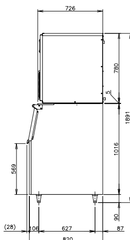
RIGHT SIDE
