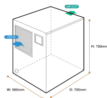
NUGGET ICE AIR SYSTEM
