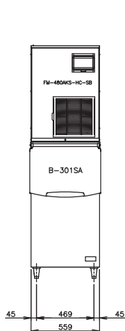
FRONT SIDE
