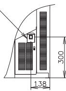
VIEW A(1/10)
