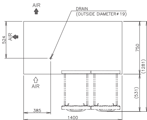
VIEW A (1/10)
