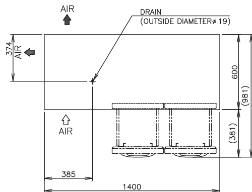
VIEW A (1/10)
