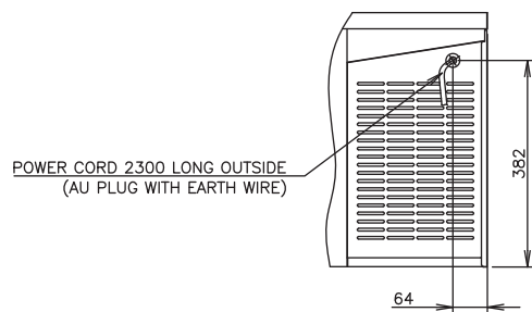
VIEW A (1/10)
