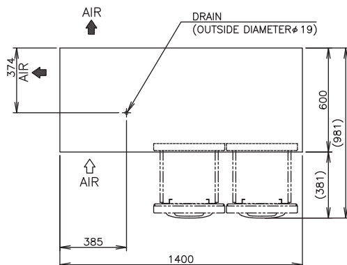
VIEW A (1/10)
