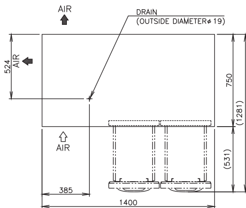
VIEW A (1/10)
