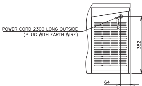
VIEW A (1/10)
