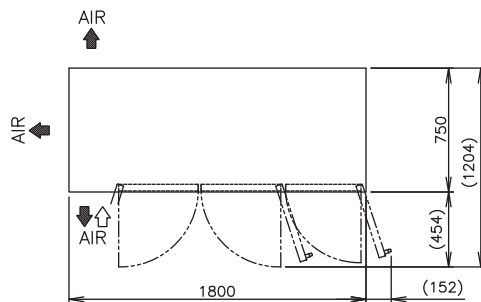
VIEW A(1/10)
