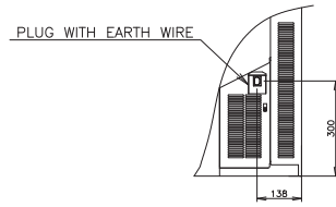
VIEW A(1/10)
